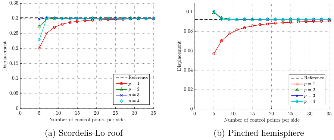
Figure 3.6: Displacement convergence of \mathbf{M} - \mathbf{N} -mixed formulation.
